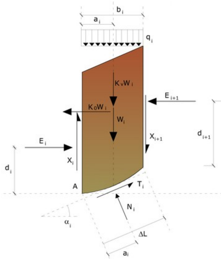
Actions on the i -the slice
