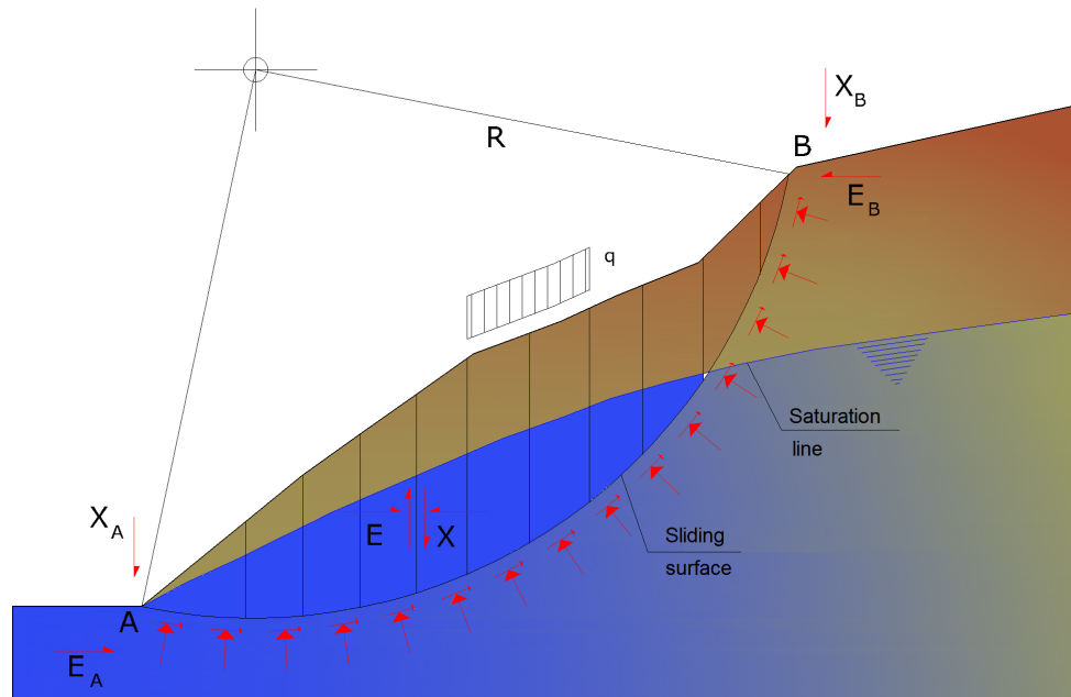
Representation of a calculation section of a slope
