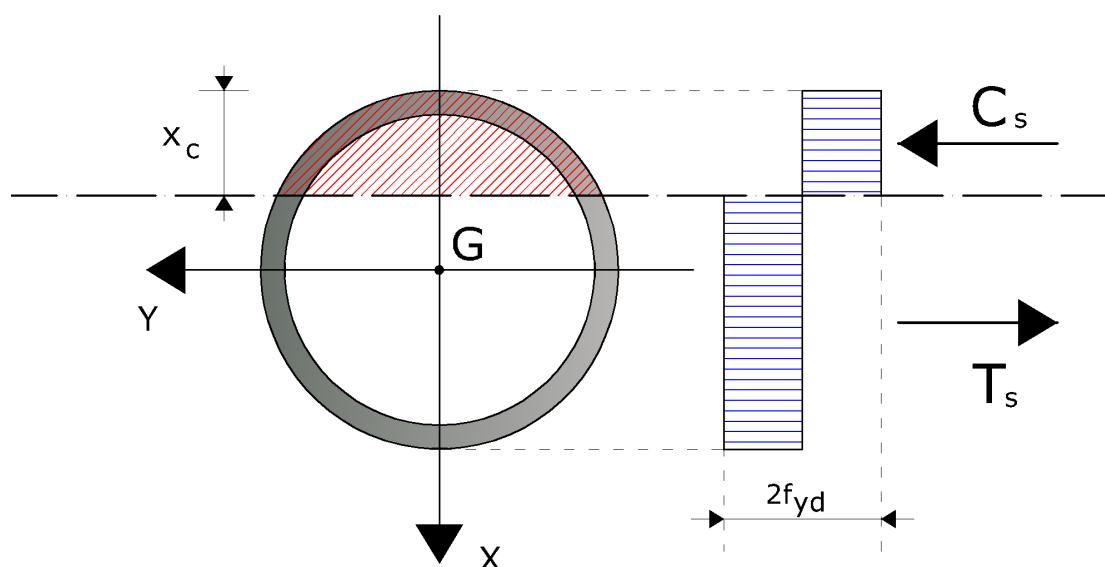
Reference diagram for the calculation of the yield moment for a steel tubular section
