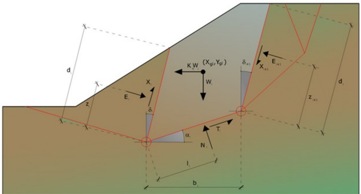
Actions on the i-th slice according to Sarma
