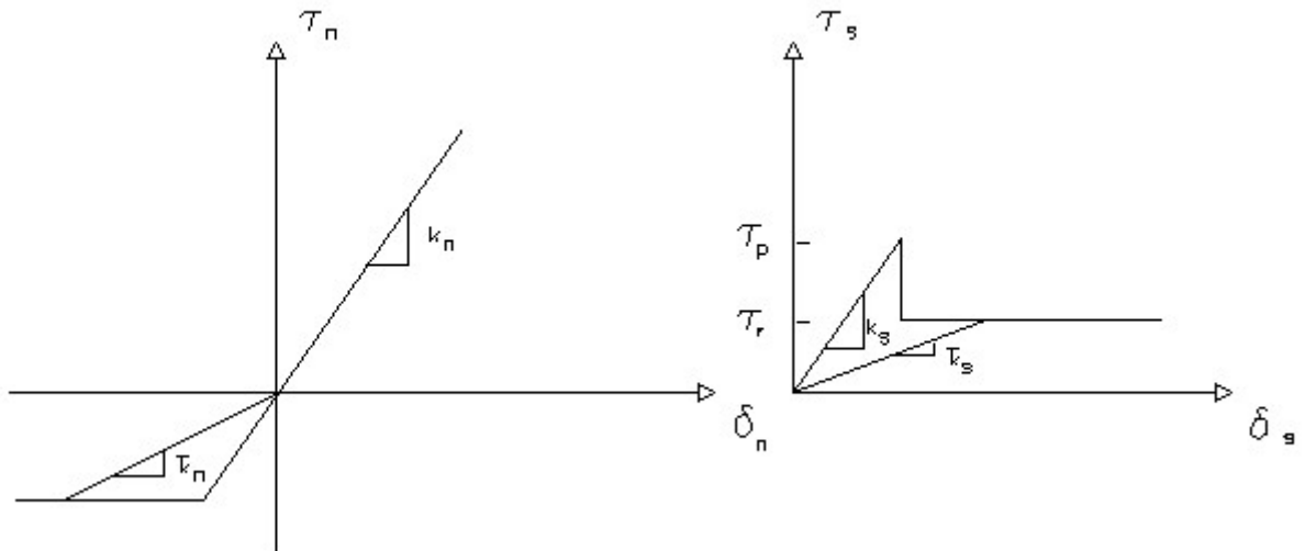
Figure 7.1.2 Secant stiffness method for obtaining \bar{k}_n \bar{k}_s
