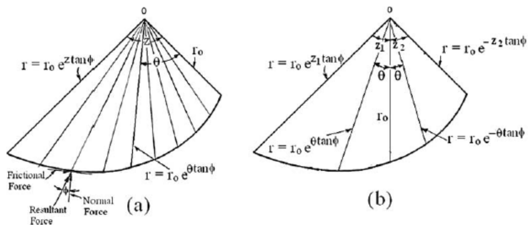
Characteristics of a logarithmic spiral
