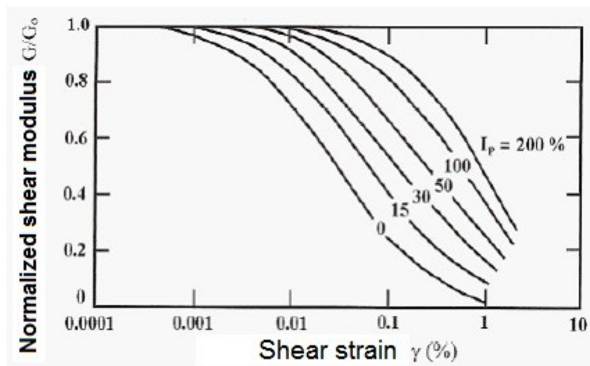
Diagram used for the calculation of the shear modulus
